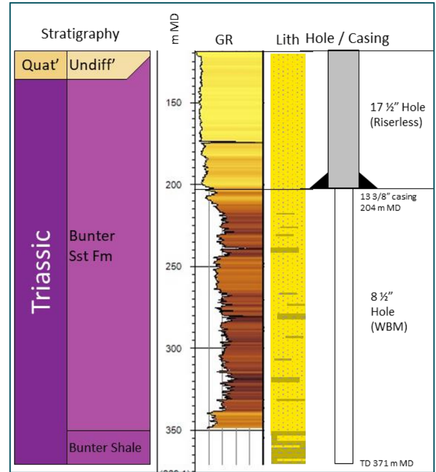
Well schematic
